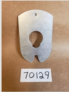
70129 - .28 Venturi Shutter (25K)
