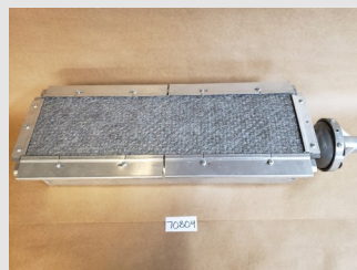
70804 - 37K Burner w/ Mat
